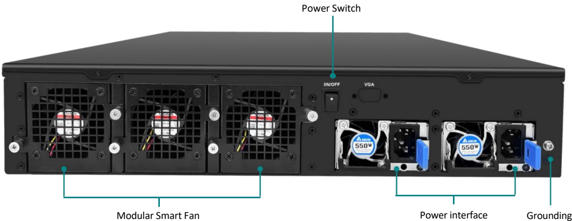
Rear View
